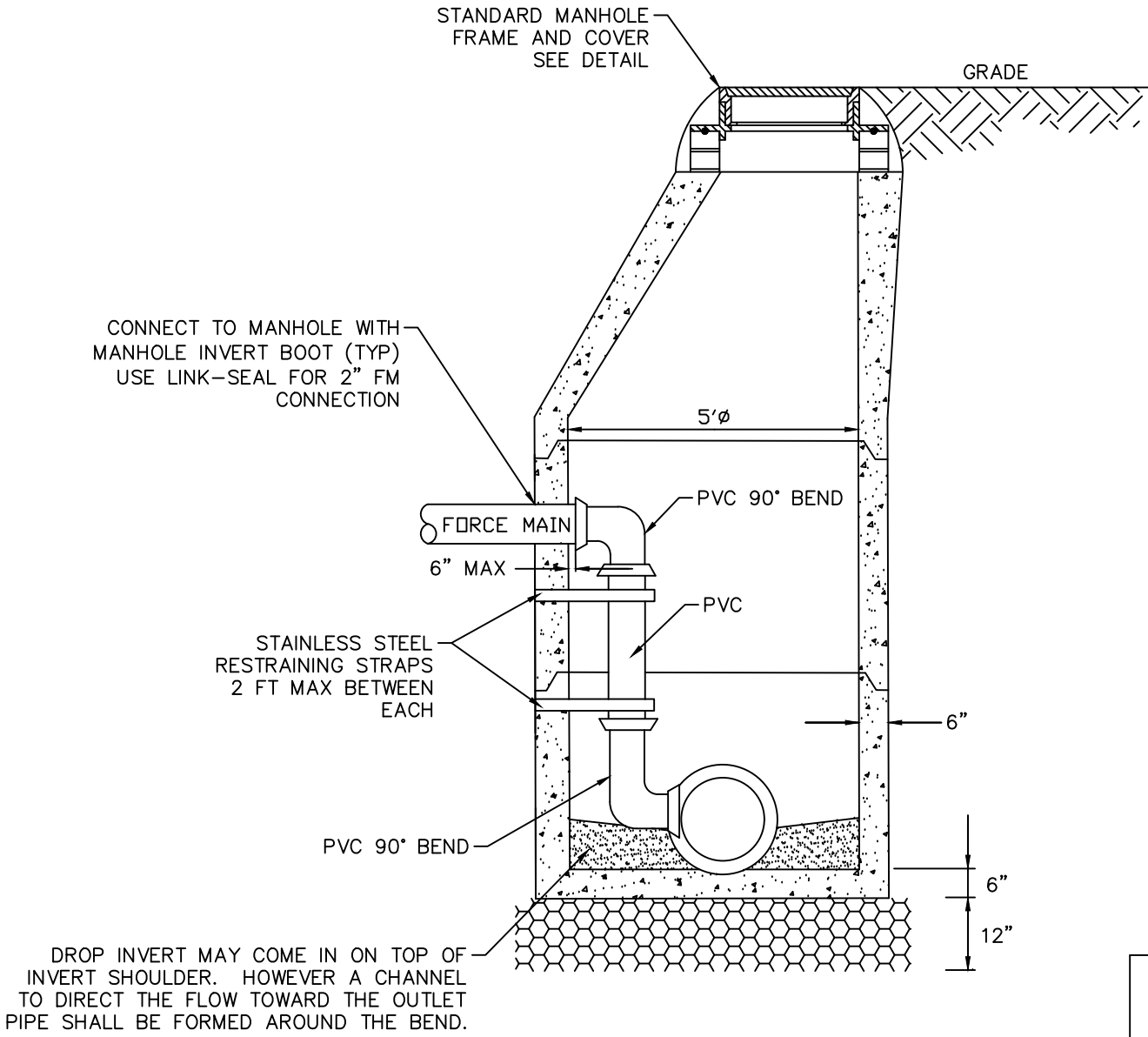
FORCE MAIN INSIDE DROP DETAIL N.T.S.
