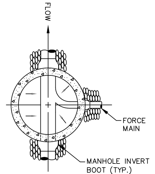
PLAN VIEW OF INVERT
